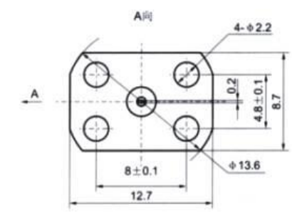
SMP-KFD-4
