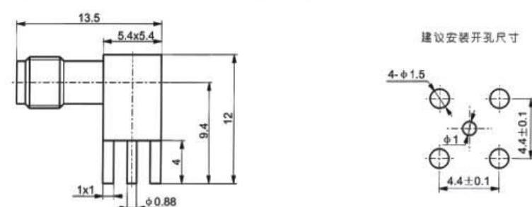
SSMA-KWHD
